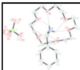
Fig. 1. The molecular structure of the title compound with the atomic numbering scheme. Displacement ellipsoids are drawn at the 30% probability level. N-bound H atoms are shown as small spheres of arbitrary radii, all other H atoms have been omitted for clarity. Dashed lines indicate N—H \cdots O hydrogen bonds.
